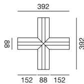
Raccordo grande per MASSA G Large joint for MASSA G Argento / Silver PMAXA2
